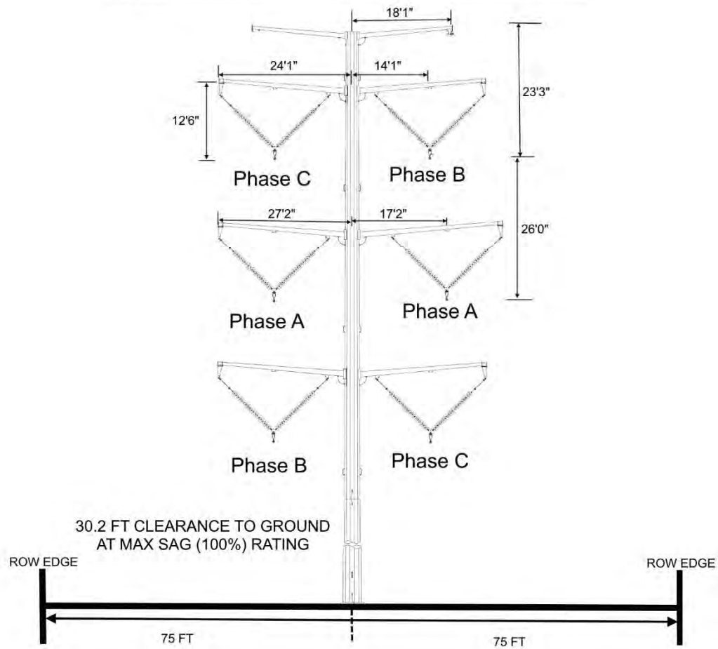
Figure 47: West Faribault – North Rochester Double Circuit
