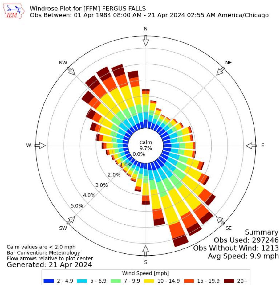
Figure 5-12 Wind Rose for Fergus Falls Municipal Airport
