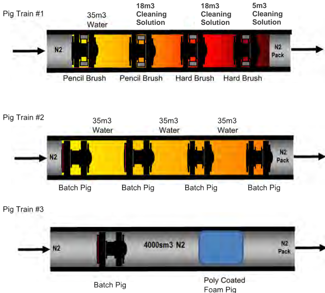
Figure 1: Cleaning validation program pig trains
