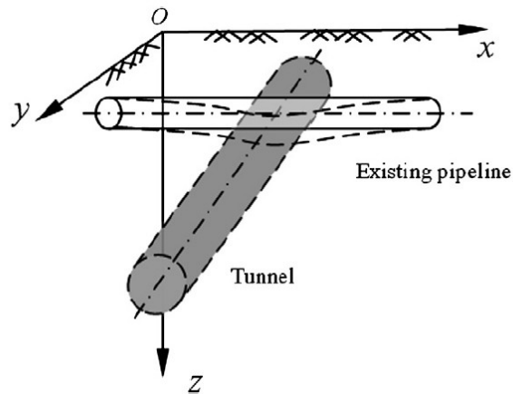
Figure 4-20: Representation of Tunneling Possible for Crossing Utility
