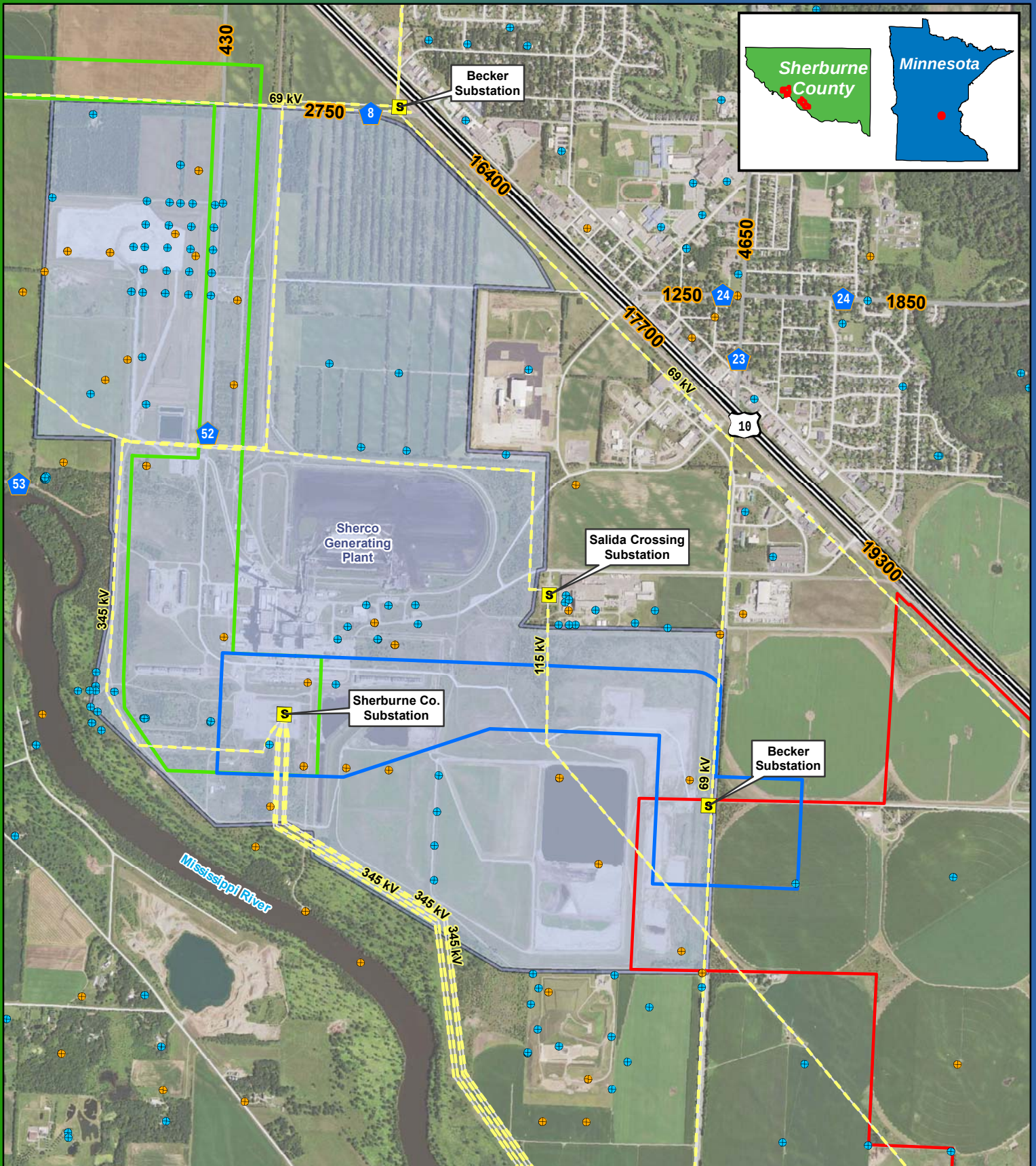
Figure 9d Existing Infrastructure and AADT (Sherco East HTVL Route) Sherco Solar Project Sherburne County, MN
