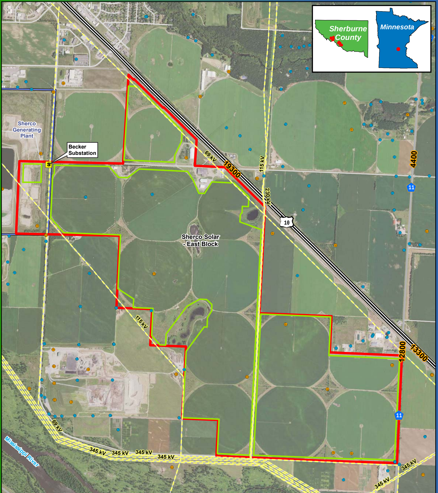
Figure 9b Existing Infrastructure and AADT (East Block) Sherco Solar Project Sherburne County, MN
