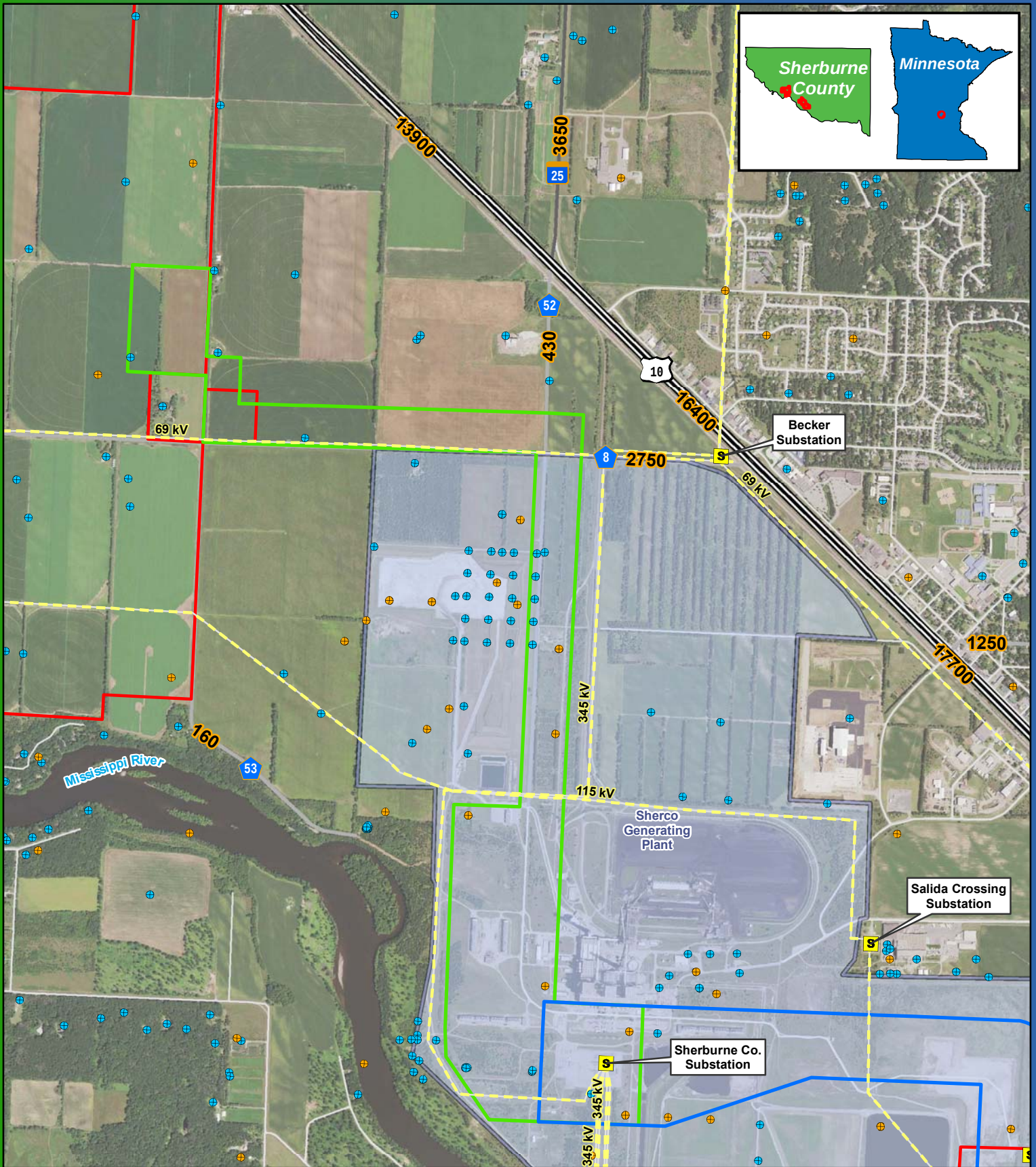
Figure 9c Existing Infrastructure and AADT (Sherco West HTVL Route) Sherco Solar Project Sherburne County, MN
