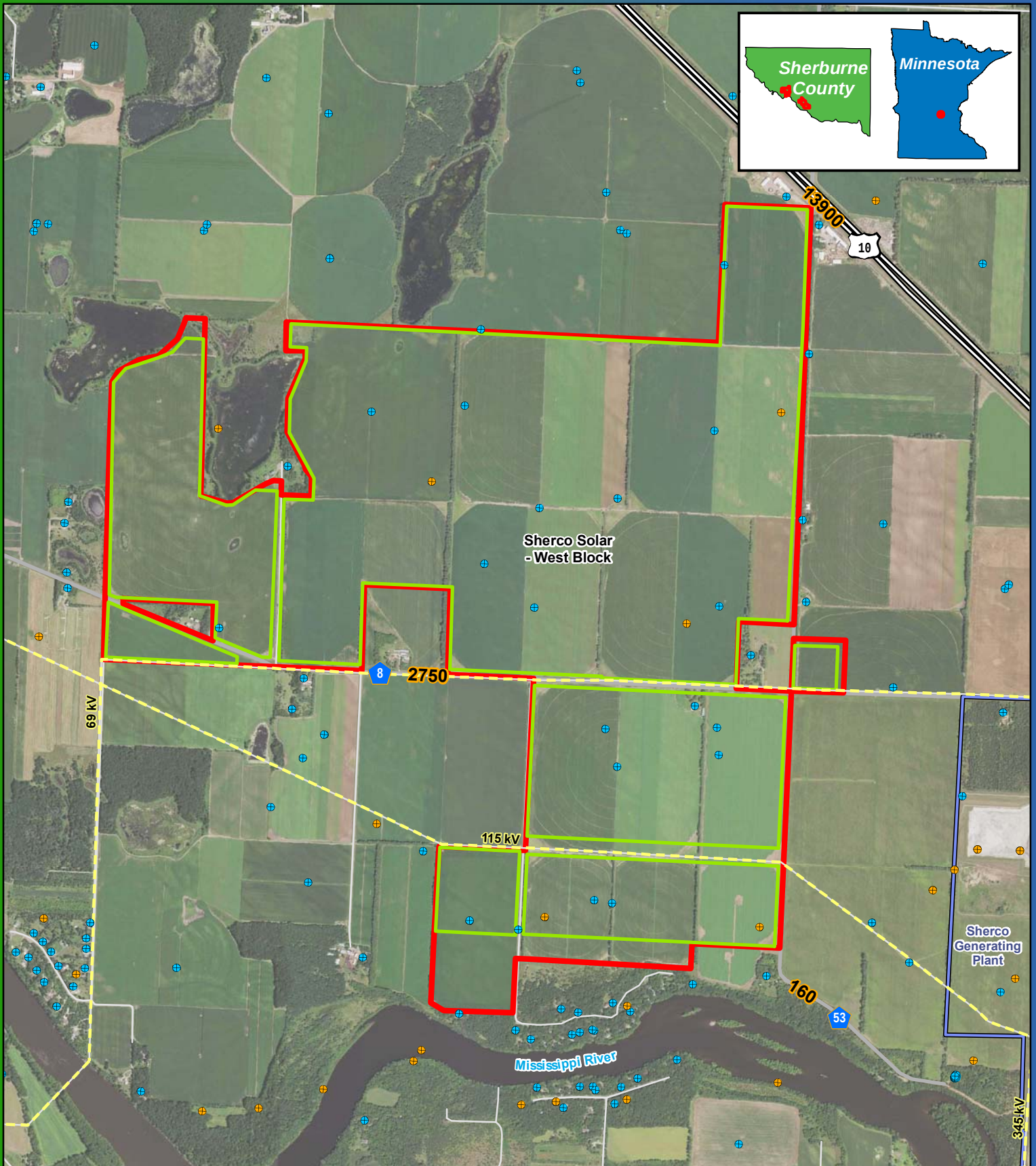
Figure 9a Existing Infrastructure and AADT (West Block) Sherco Solar Project Sherburne County, MN
