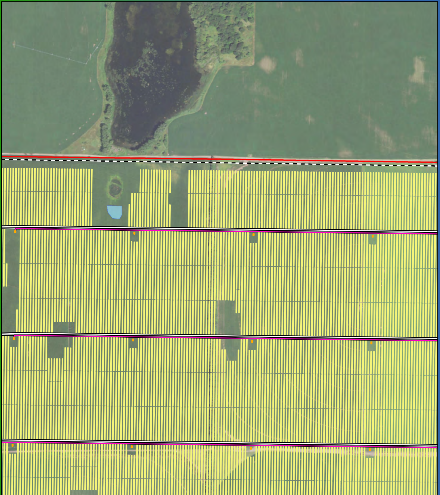
Figure 5b Detailed Preliminary Project Layout Sherco Solar Project Sherburne County, MN
