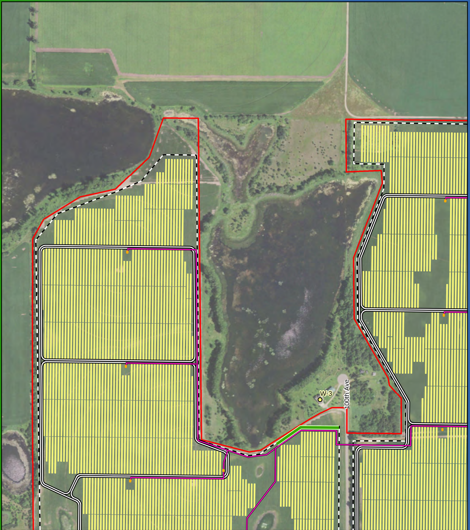
Figure 5a Detailed Preliminary Project Layout Sherco Solar Project Sherburne County, MN
