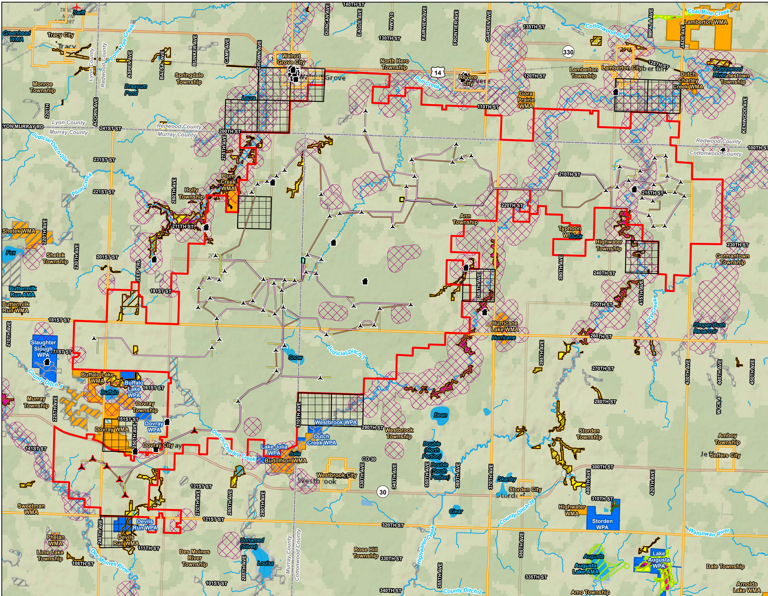
Figure 10a Unique Natural Features Vestas V162
