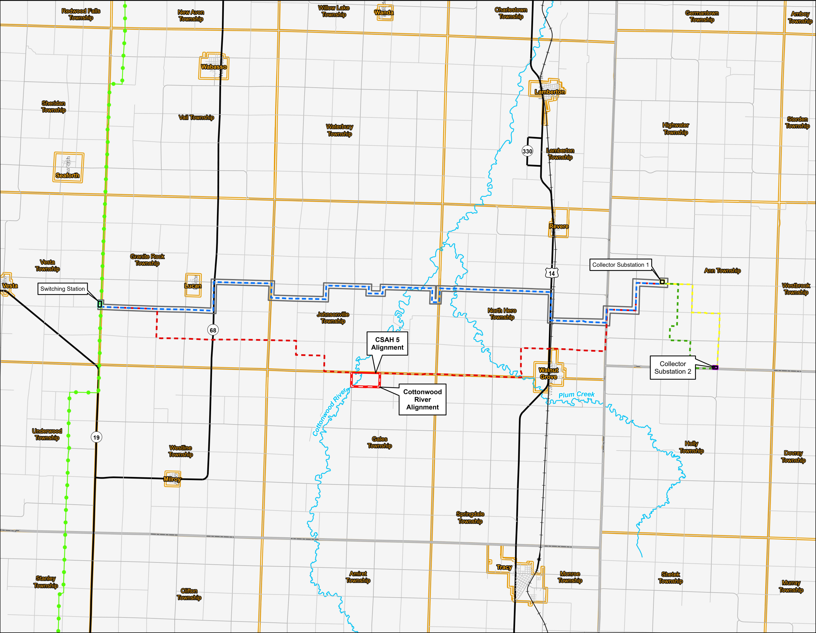
Figure 2 Project Location (HVTL) Plum Creek Wind Project Redwood, Murray, and Cottonwood Counties, MN
