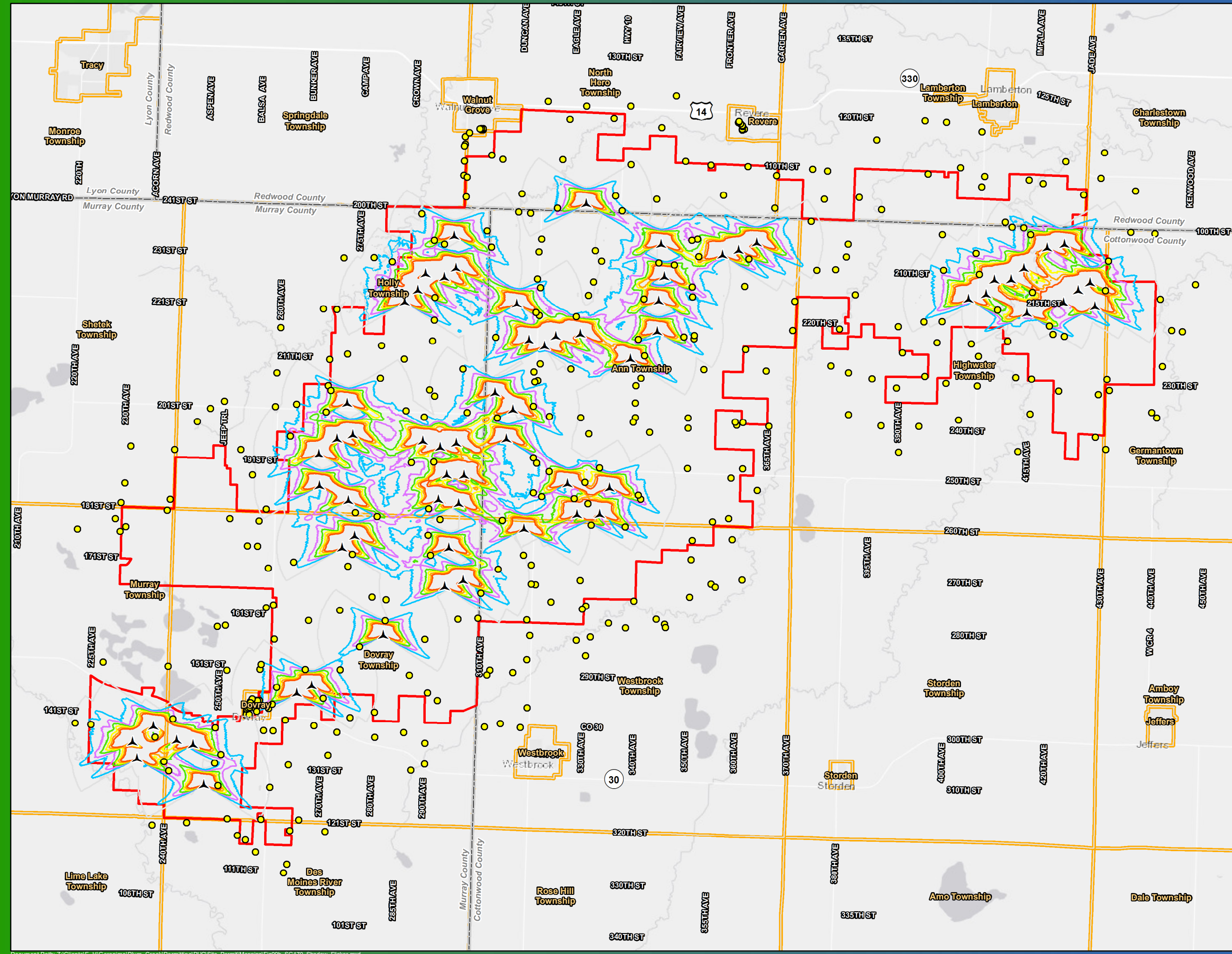
Figure 9b Shadow Flicker Siemens Gamesa SG170 Plum Creek Wind Project Redwood, Murray, and Cottonwood Counties, MN
