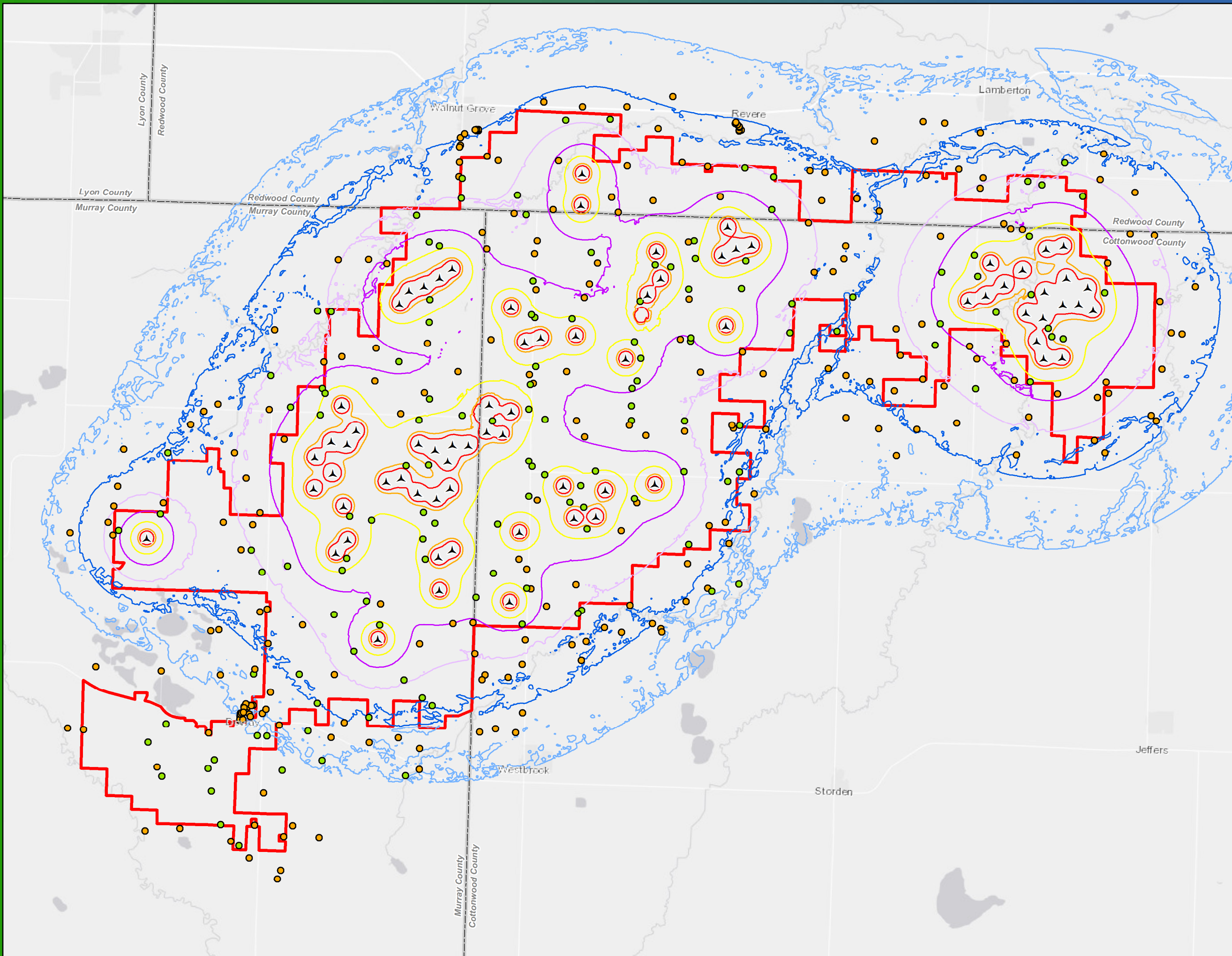
Figure 7a Sound/Noise Vestas V162 Plum Creek Wind Project Redwood, Murray, and Cottonwood Counties, MN
