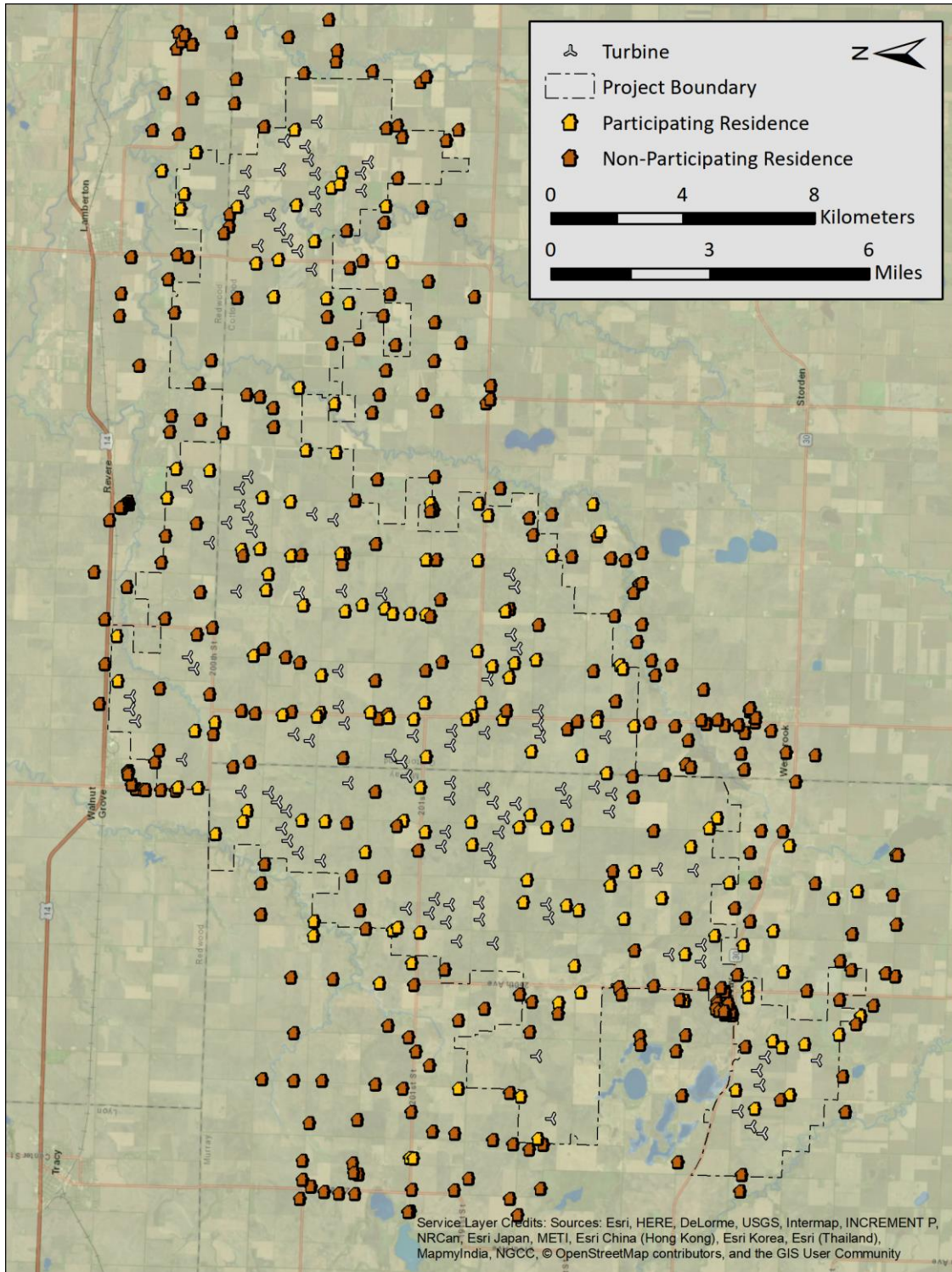
FIGURE 2: PLUM CREEK WIND FARM SITE MAP WITH GE LAYOUT
