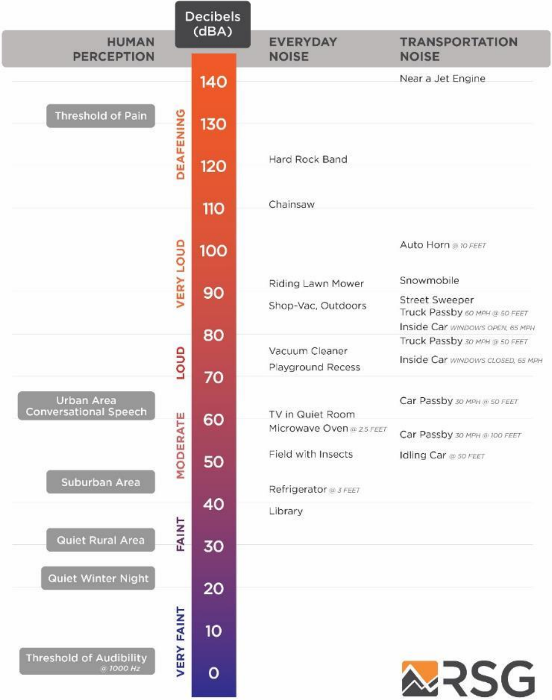
FIGURE 36: A SCALE OF SOUND PRESSURE LEVELS FOR TYPICAL SOUND SOURCES
