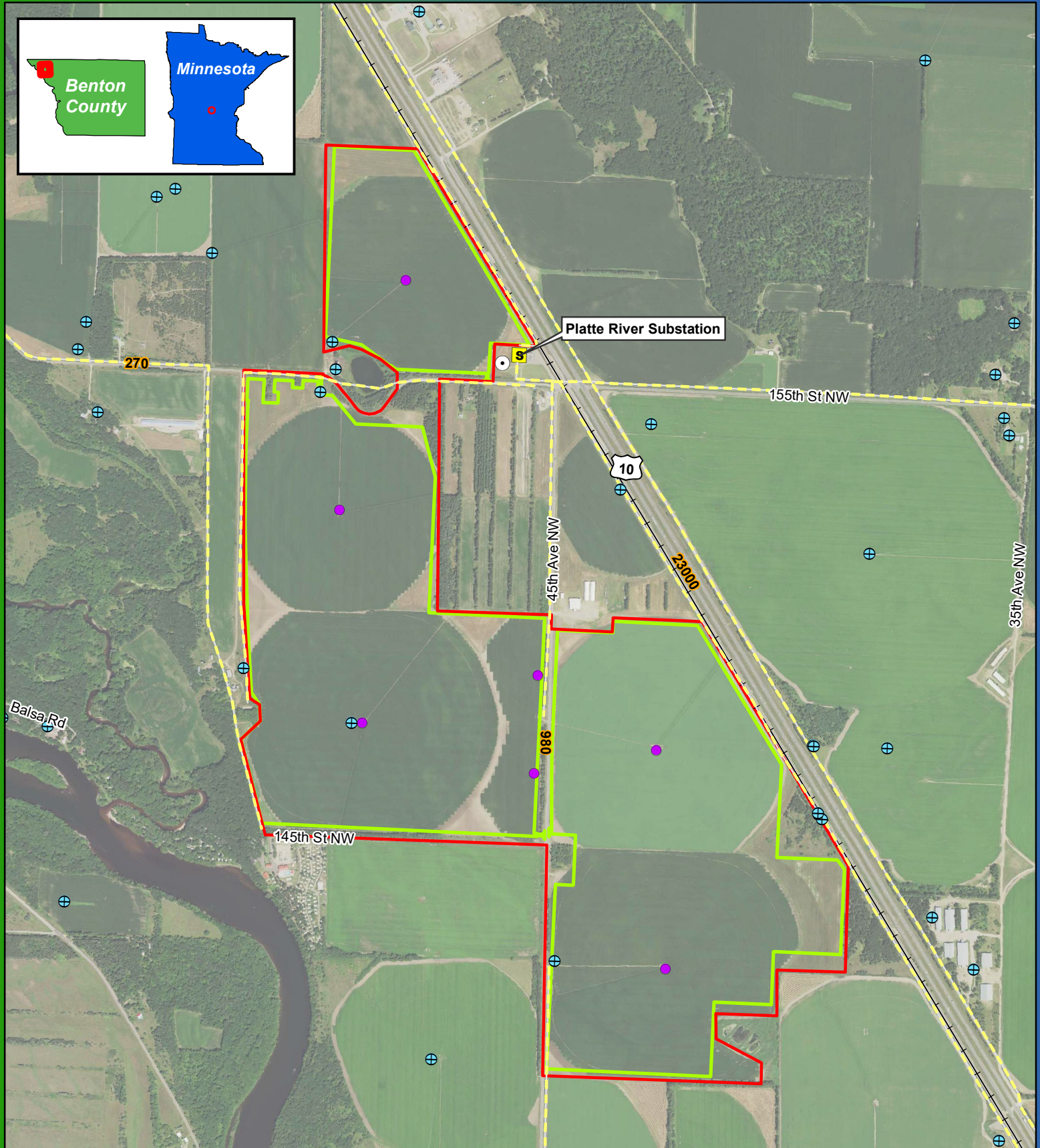
Figure 9 Existing Infrastructure and AADT Regal Solar Project Benton County, MN 45.783906, -94.261881
